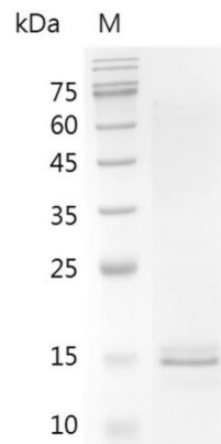
SDS-PAGE analysis of recombinant H/M/R Activin A, tag free
