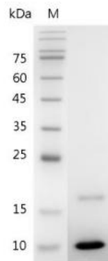
SDS-PAGE analysis of recombinant mouse IGF-I
