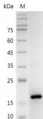
SDS-PAGE analysis of recombinant mouse CD27L
