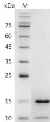
SDS-PAGE analysis of recombinant human BMP14
