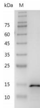
SDS-PAGE analysis of recombinant human TWEAK
