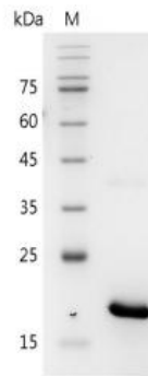
SDS-PAGE analysis of recombinant mouseIL-17B
