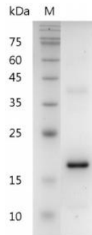
SDS-PAGE analysis of recombinant human IL-37
