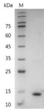
SDS-PAGE analysis of recombinant mouse IL-31
