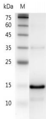
SDS-PAGE analysis of recombinant human IL-21
