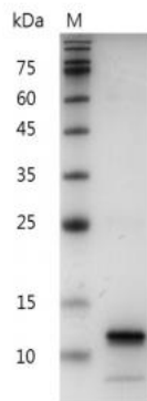
SDS-PAGE analysis of recombinant swine CXCL10
