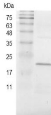
SDS-PAGE analysis of recombinant swine CCL2
