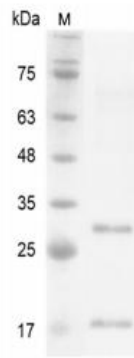
SDS-PAGE analysis of recombinant human IL- 17D
