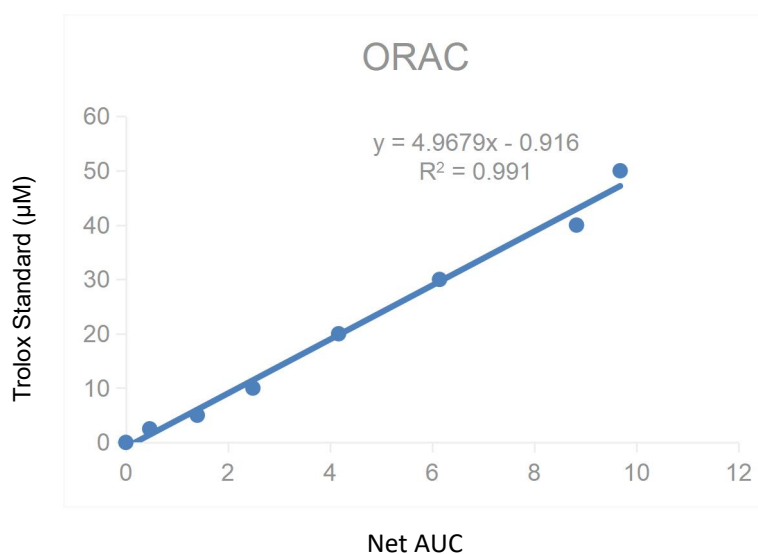
Figure 1. Standard curve for ORAC.
