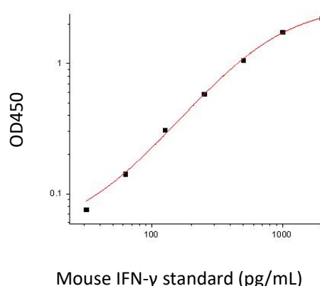
Fig.1. Standard Curve of Mouse IFN- \gamma in 96-well plate assay, data provided for demonstration purposes only. A new standard Curve must be generated for each assay.
