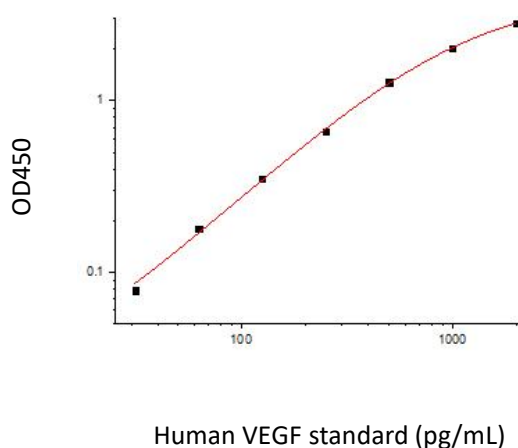
Fig.1. Standard Curve of Human VEGF in 96-well plate assay, data provided for demonstration purposes only. A new standard Curve must be generated for each assay.
