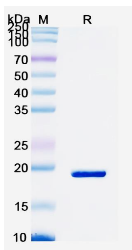
SDS-PAGE for Recombinant Mouse SOX9 Protein
