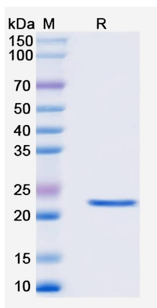
SDS PAGE for Recombinant Human TPO protein
