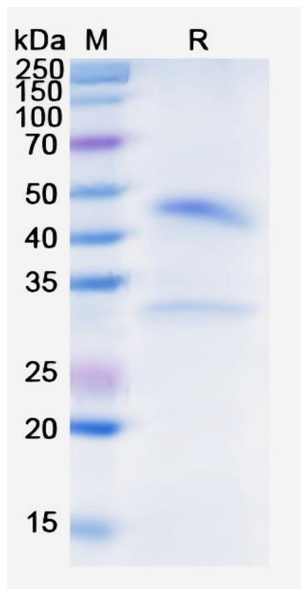
SDS PAGE for Recombinant Human MUC2 Protein
