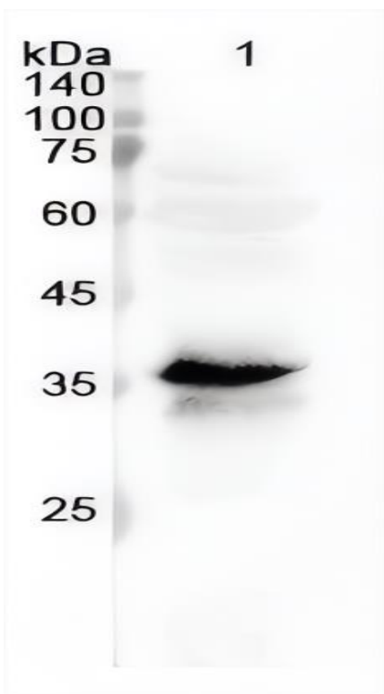
Western blot
