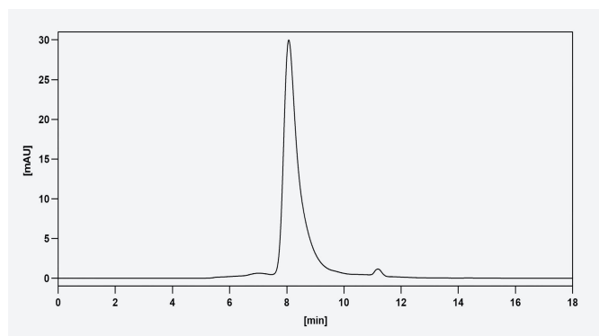
SEC-HPLC
