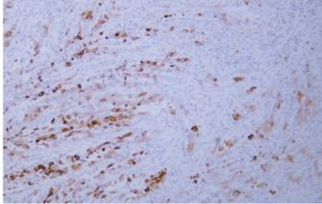
Fig. Human colon carcinoma tissue was stained with Anti-COX-2 Antibody.
